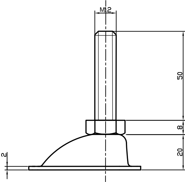
S-L M12X50
